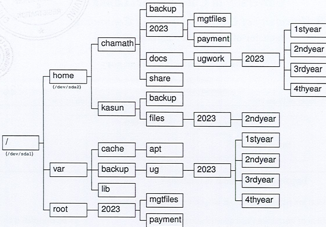
Figure 1: Extract of an Ubuntu GNU/Linux directory structure
